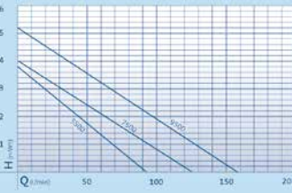
Aquarius Fountain Set 5'500 – 9'500
